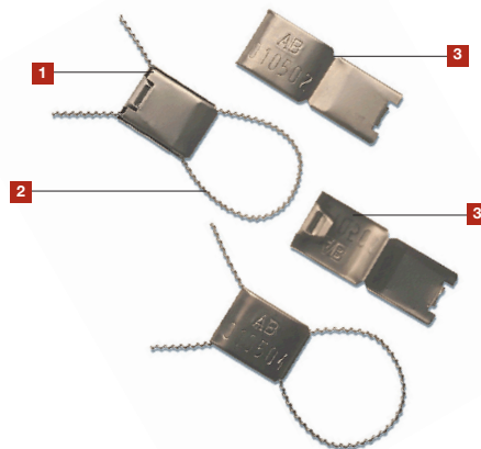
METAL CLIP SEAL
